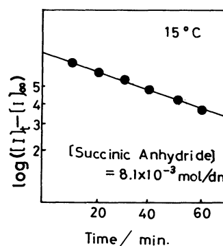
Fig. 3. First-order plot for the reaction of Ni(bpy)(cod) with succinic anhydride.
